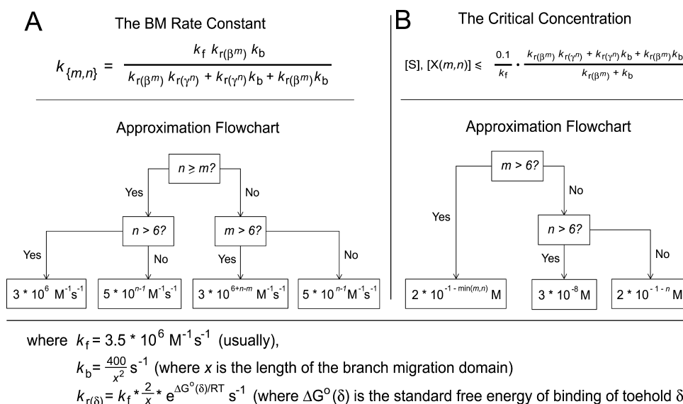
Figure 8. (A) Flowchart for order of magnitude estimate of k_{\{m,n\}} . This flowchart assumes average binding strength and no secondary structure and approximates the rate constant at 25 °C and 11.5 mM \text{Mg}^{2+} or 1 M \text{Na}^+ . (B) Flowchart for estimating the critical concentration, below which the BM rate constant ( k_{\{m,n\}} ) accurately predicts kinetics.
